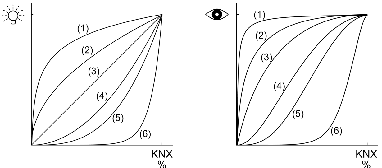
Image 5: Dimming characteristics in the value range
