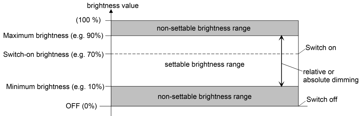
Image 11: Example of a brightness range with minimum brightness
