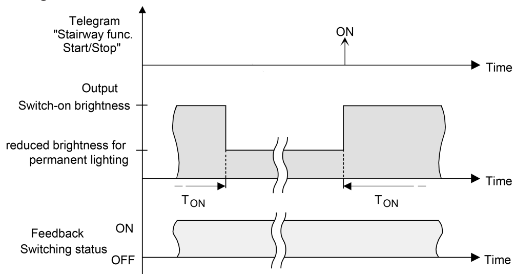
Image 21: The continuous lighting of the staircase function without soft functions
