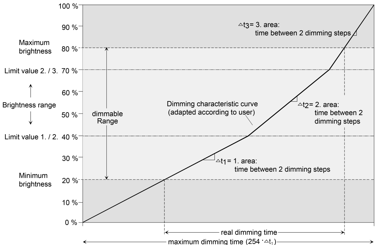
Image 9: User-defined dimming characteristic as an example with minimum brightness and
