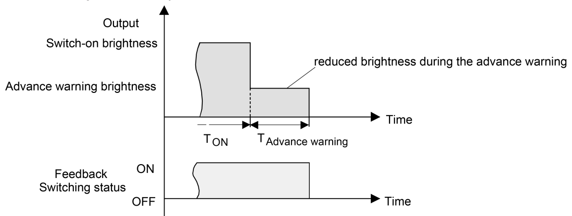
Image 19: The pre-warning function of the staircase function without soft OFF function
