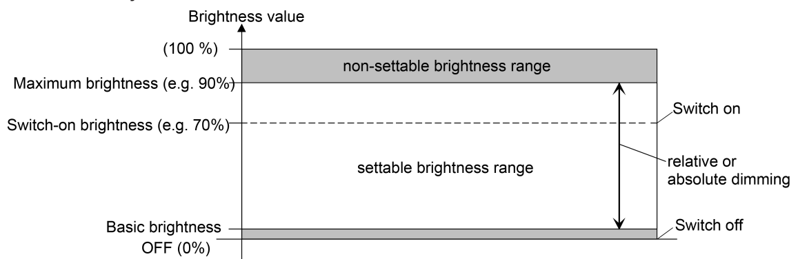
Image 10: Example of a brightness range with basic brightness
