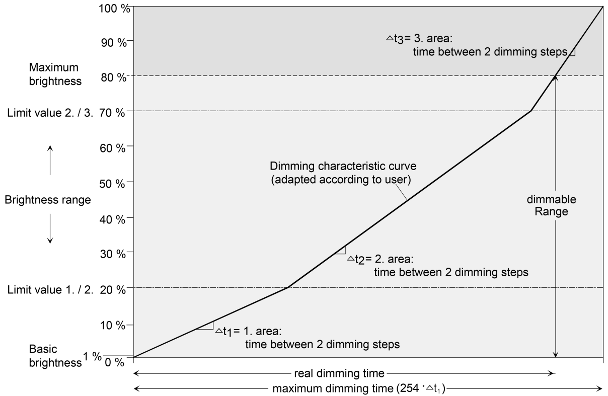
Image 8: User-defined dimming characteristic as an example with basic brightness and maximum brightness
