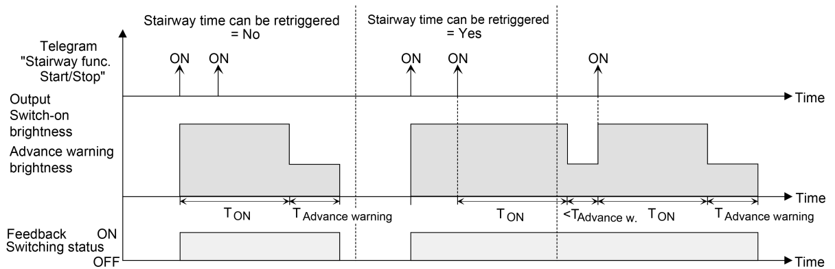
Image 15: Switch-on behaviour of the staircase function without soft functions
