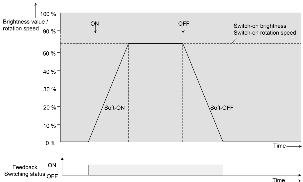
Image 13: Dimming behaviour of the soft ON/OFF functions (as an example)
