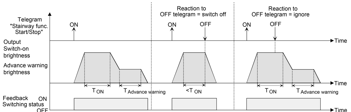
Image 18: Switch-off behaviour of the staircase function with soft functions (as an example with minimum brightness = 0 %)
