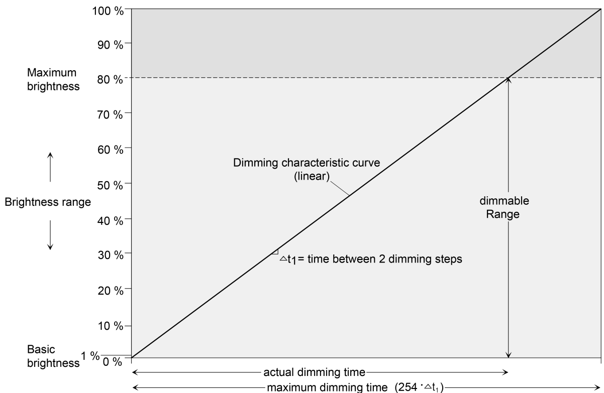
Image 6: Linear dimming characteristic as an example with basic brightness and maximum brightness
