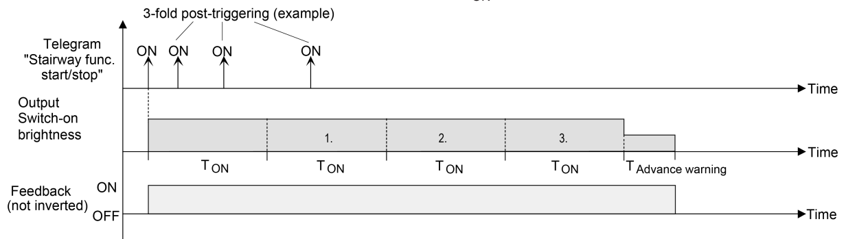
Image 23: Time extension of the staircase function
