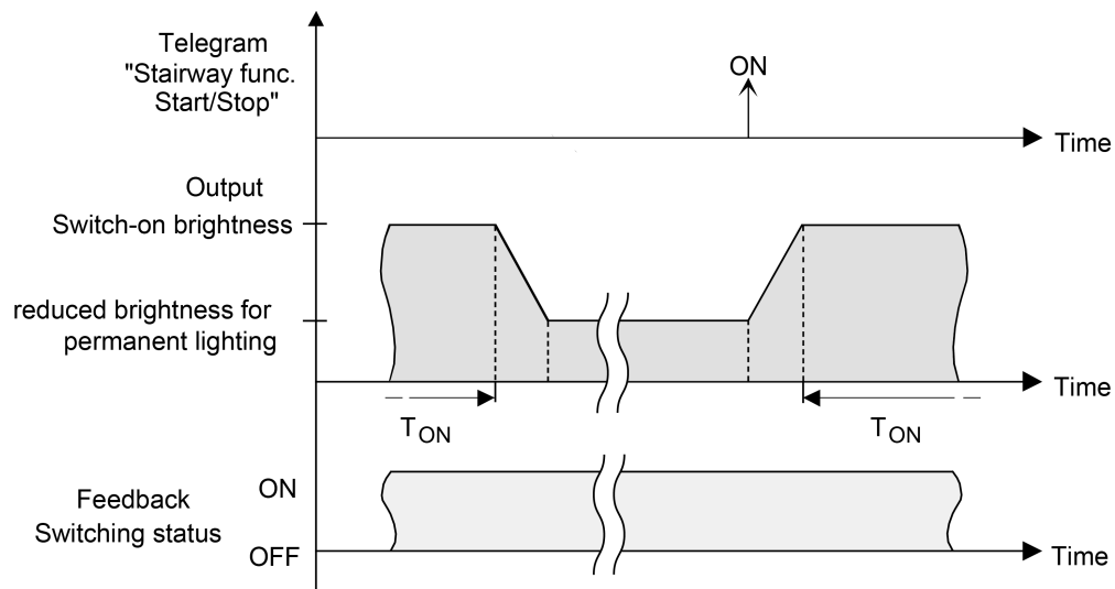
Image 22: The continuous lighting of the staircase function with soft OFF functions
