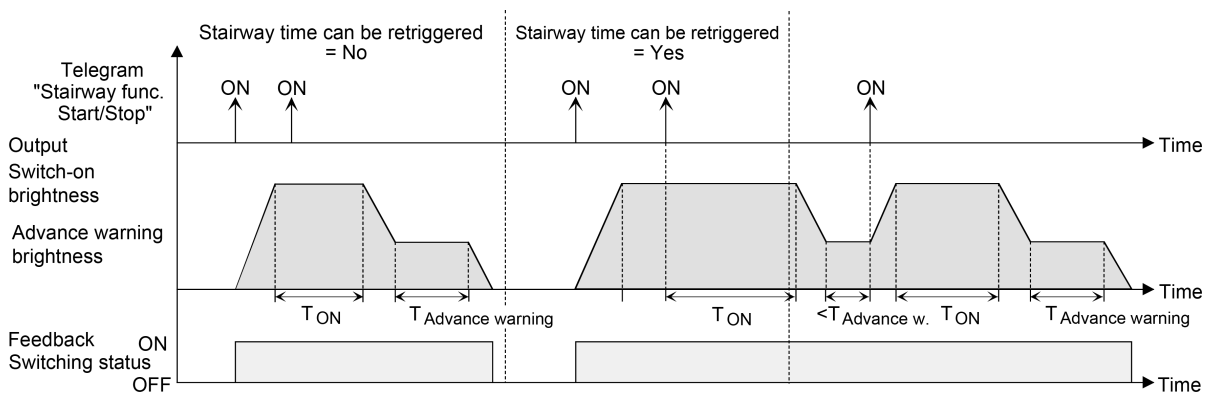
Image 16: Switch-on behaviour of the staircase function with soft functions (as an example with minimum brightness = 0 %)
