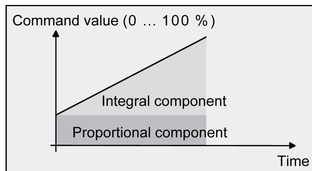
Figure 20: Continuous PI control
