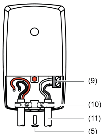
Figure 7: Connection of an external contact / remote sensor
