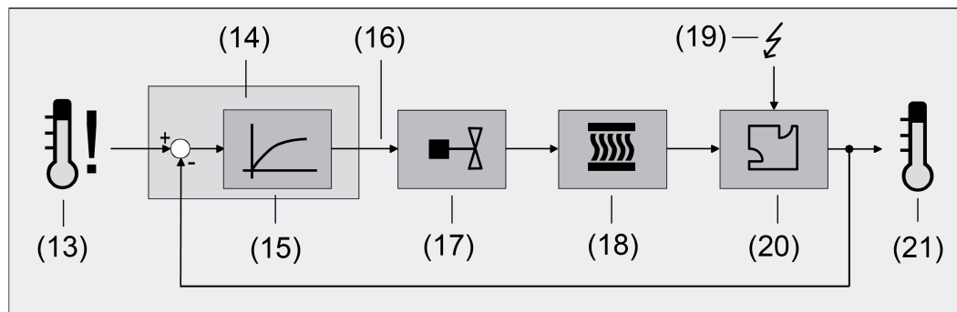
Figure 19: Controlled system of single-room temperature control
