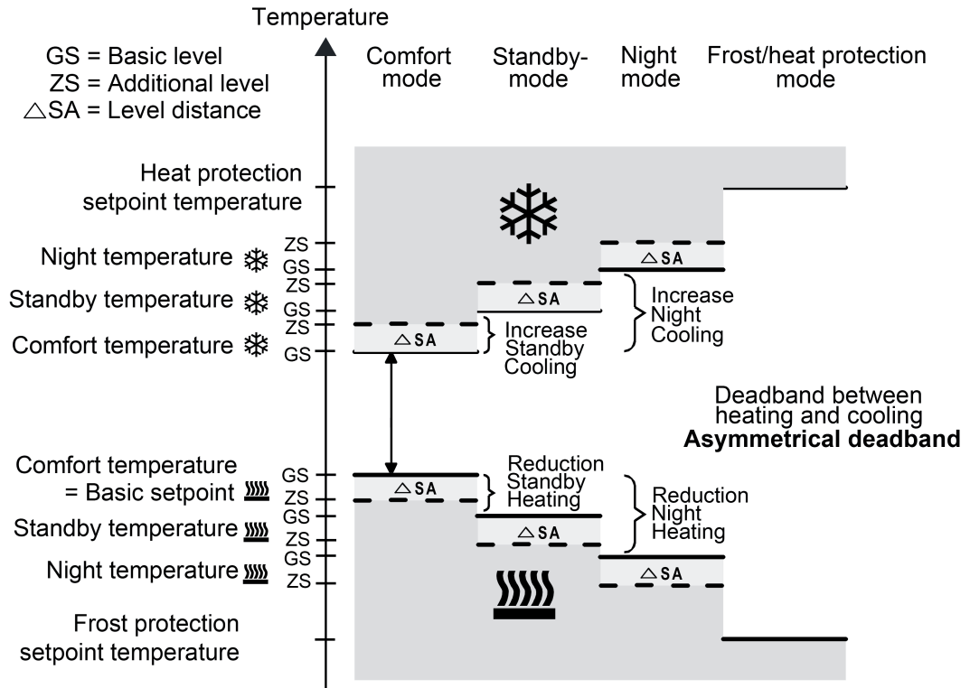
Figure 39: Setpoint temperatures in the operating mode "Basic and additional heating and cooling" with asymmetrical deadband
