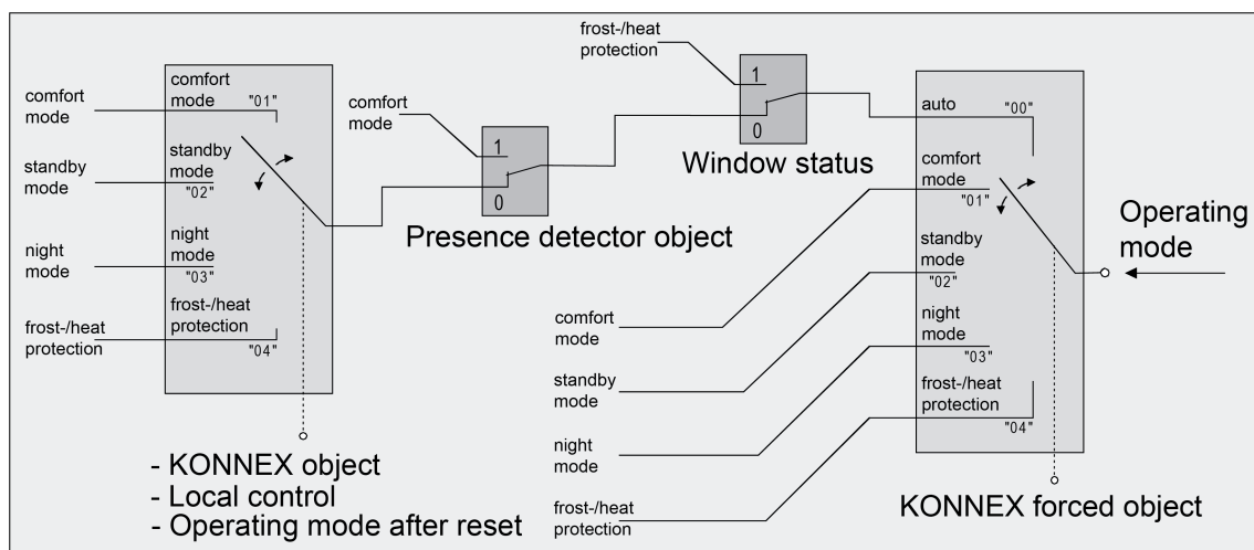
Figure 31: Operating mode change-over through KNX object with presence detector
