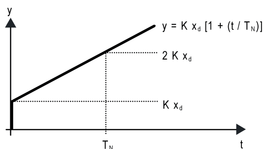
Figure 26: Function of the command value of a PI control
