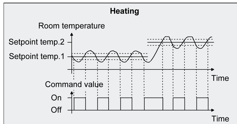
Figure 22: 2-point feedback control for the single "Heating" operating mode
