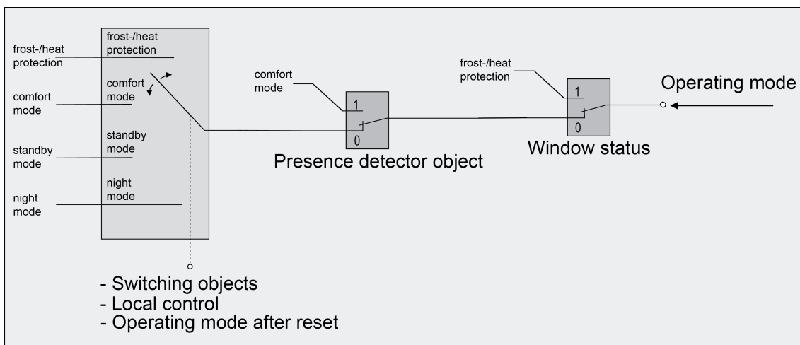
Figure 29: Operating mode change-over through 4 x 1-bit objects with presence detector
