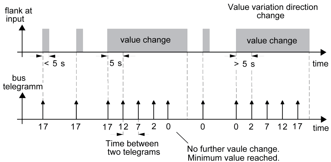
Figure 17: Example to change the value for dimming value transmitter
