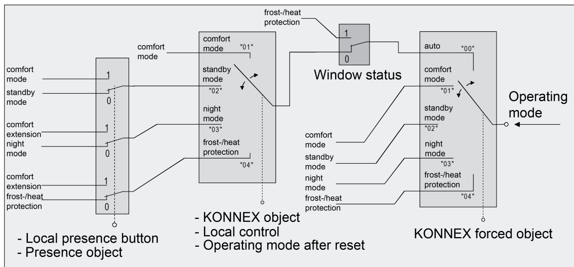
Figure 30: Operating mode change-over through KNX object with presence button
