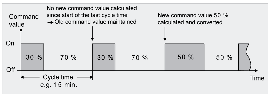
Figure 21: Switching PI control
