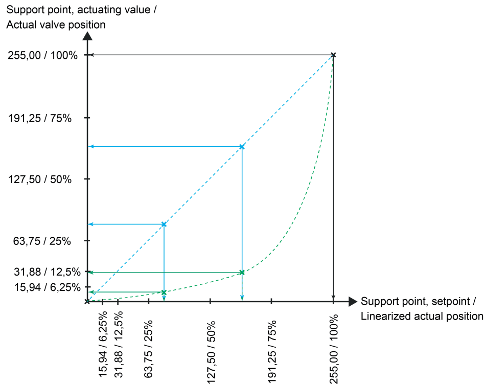
Figure 13: Characteristic curve diagram (fictitious) for the "Actual position" object
