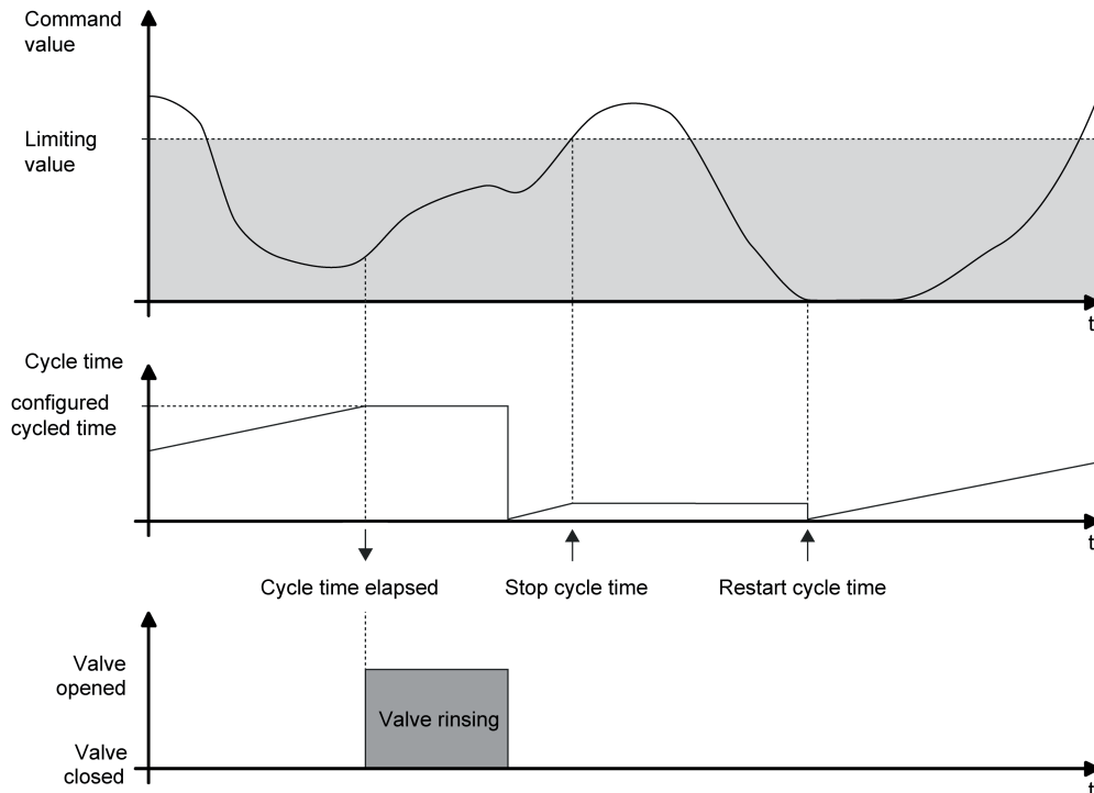
Figure 14: Example of a minimum command value limiting value for intelligent valve rinsing
