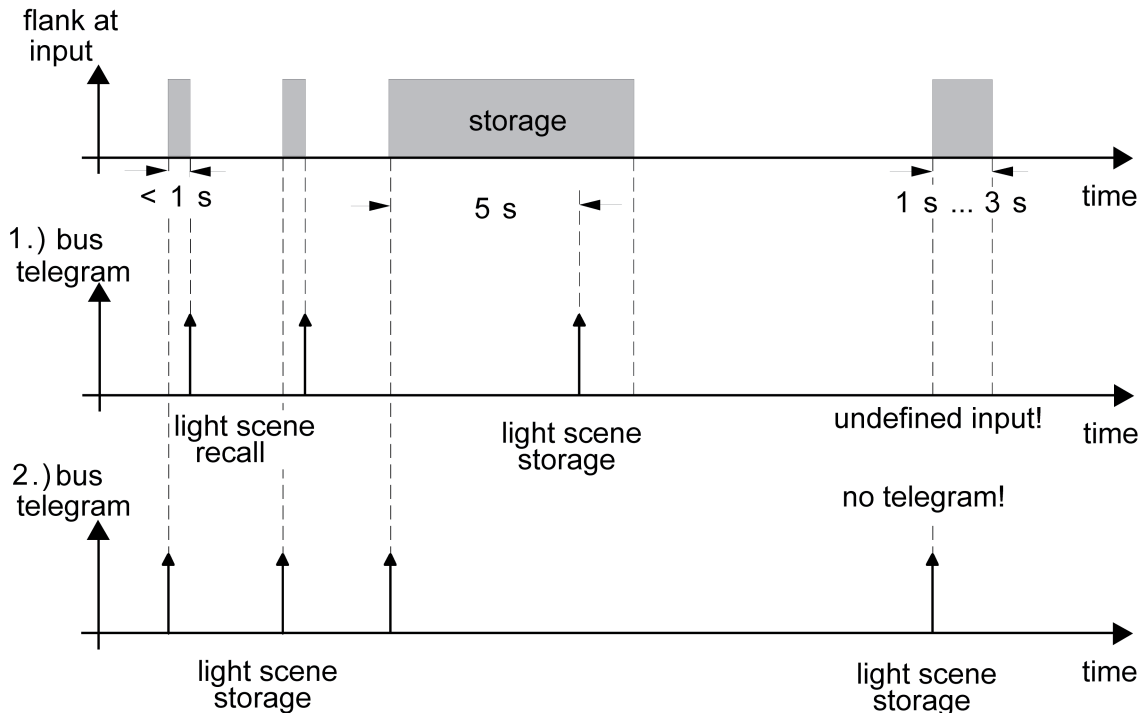
Figure 18: Example of scene storage
