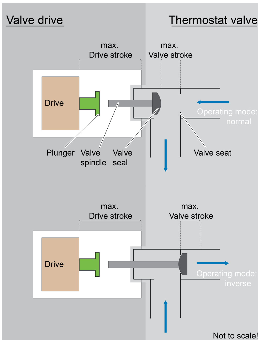
Figure 9: Principle sketch of the functional unit
