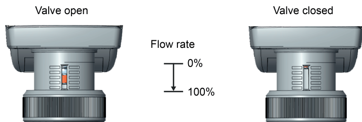
Figure 11: Inverse (command value 0% -> valve open)
