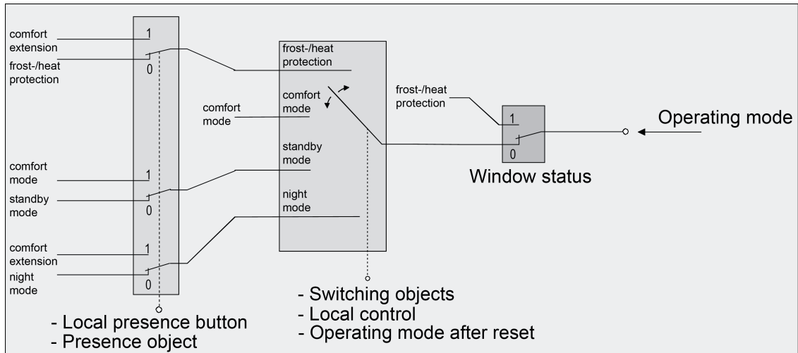
Figure 28: Operating mode change-over through 4 x 1-bit objects with presence button
