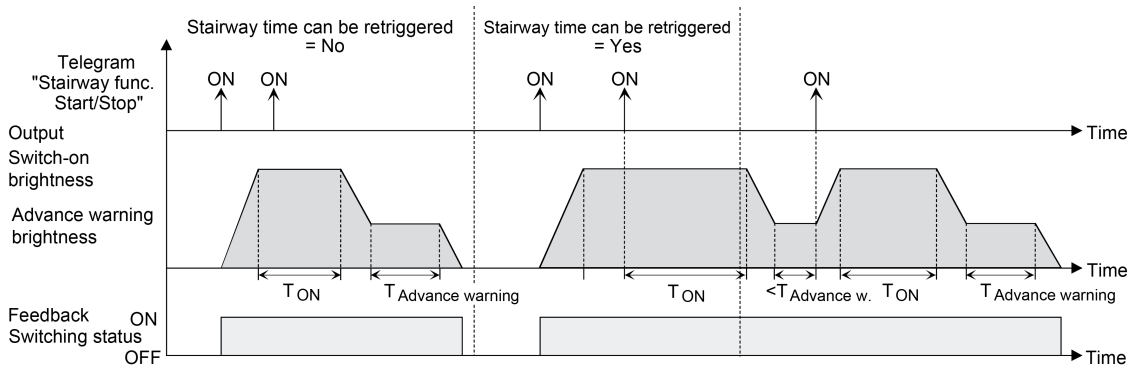
Figure 22: Switch-on behaviour of the staircase function with soft functions (for example with minimum brightness = 0 %)
