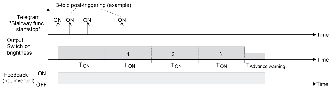
Figure 29: Time extension of the staircase function
