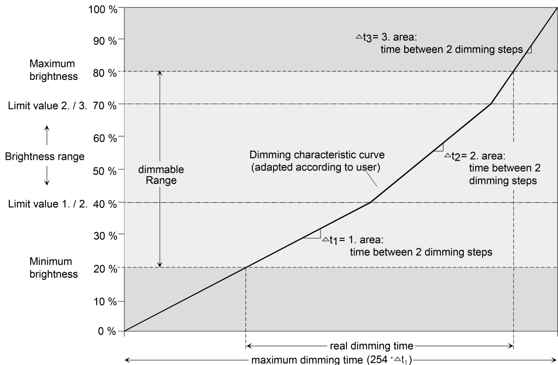
Figure 18: User-defined dimming characteristic as an example with minimum brightness and maximum brightness (example with 3 areas)
