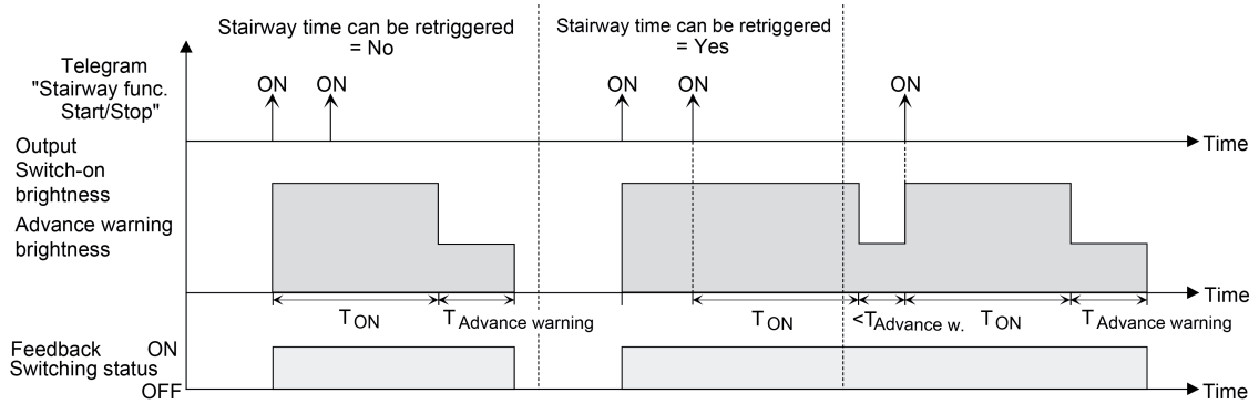
Figure 21: Switch-on behaviour of the staircase function without soft functions
