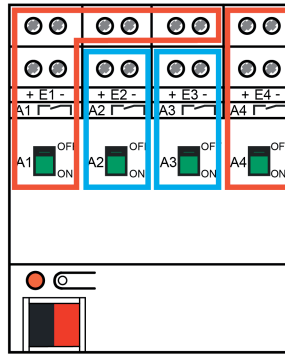
Figure 8: Configuration 5 - Inputs 1...3 affect output 1 / Input 4 affects output 4 / Outputs 2 and 3 can be used independently
