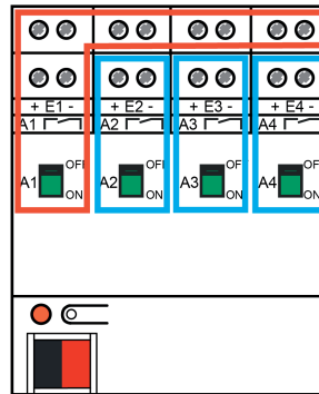
Figure 5: Configuration 2 - All 4 inputs affect output 1 / Outputs 2...4 can be used independently
