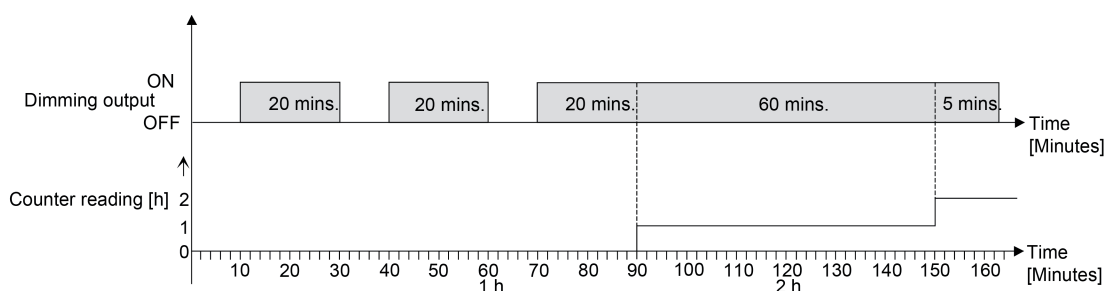
Figure 37: Function of the operating hours counter (using the example of an up-counter)
