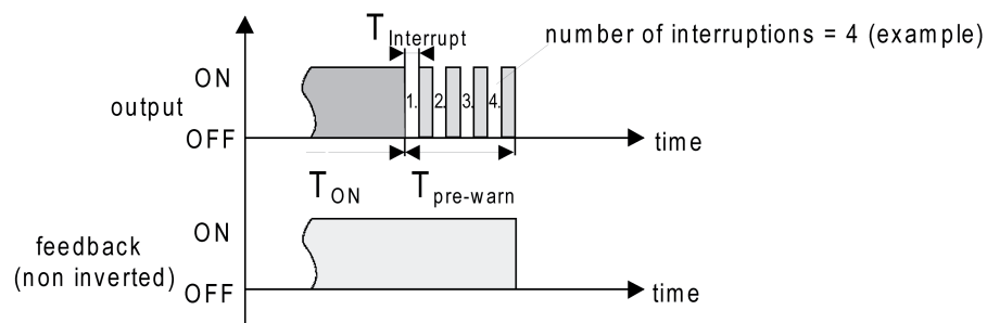
Figure 34: The pre-warning function of the staircase function (example)
