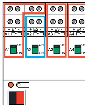
Figure 6: Configuration 3 - Inputs 1 & 2 affect output 1 / inputs 3 & 4 affect outputs 3 & 4 separately / output 2 can be used independently
