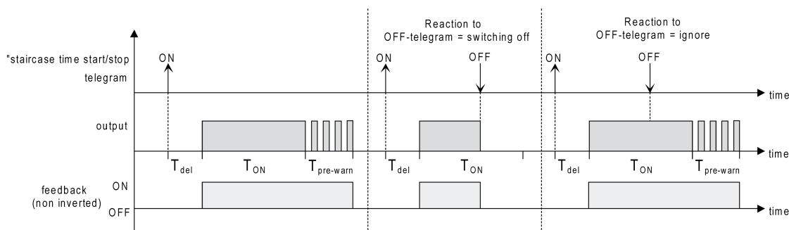
Figure 33: Switch-off behaviour of the staircase function
