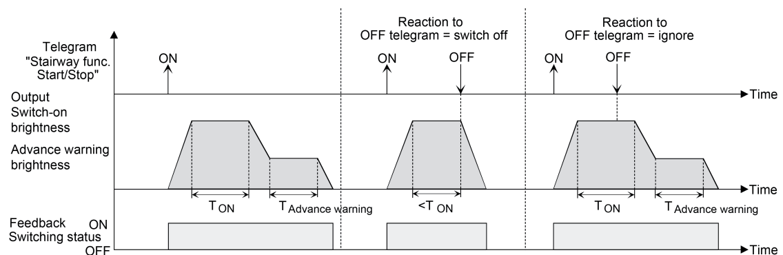
Figure 24: Switch-off behaviour of the staircase function with soft functions (for example with minimum brightness = 0 %)
