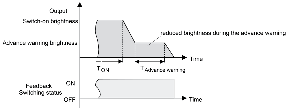
Figure 26: The pre-warning function of the staircase function with soft OFF function (for example with minimum brightness = 0 %)
