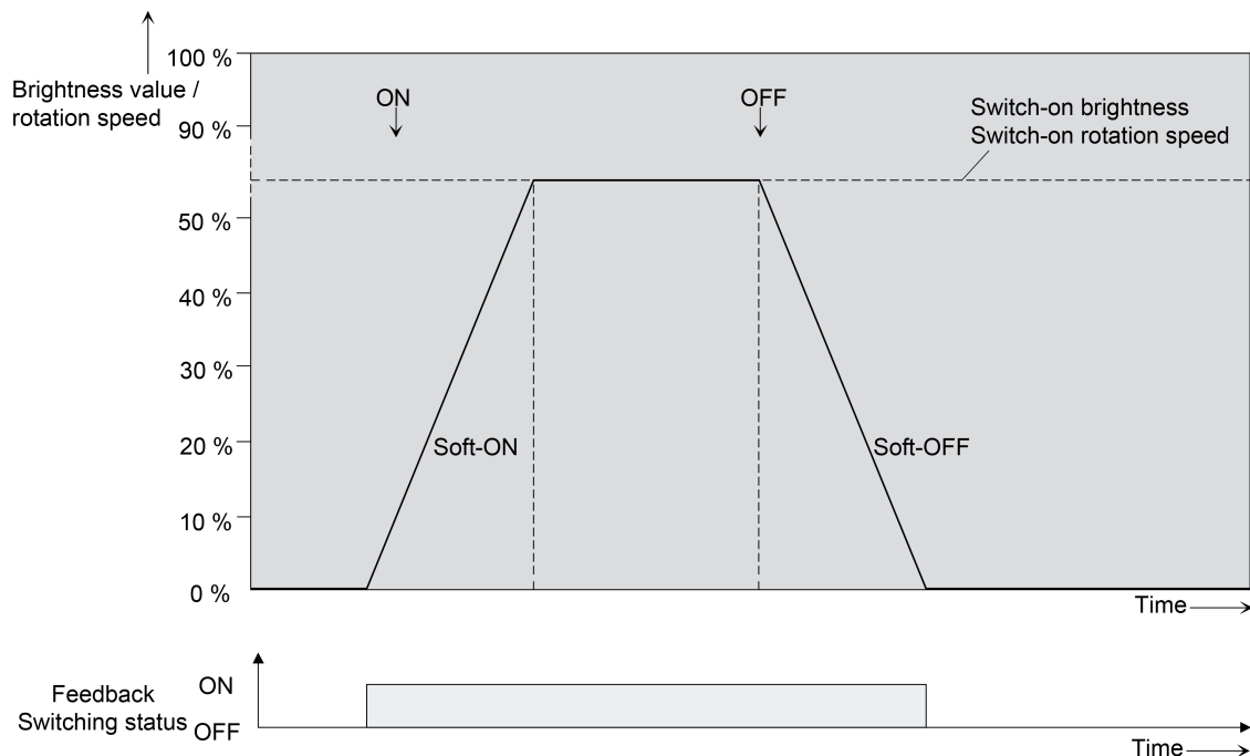
Figure 19: Dimming behaviour of the soft ON/OFF functions (as an example)
