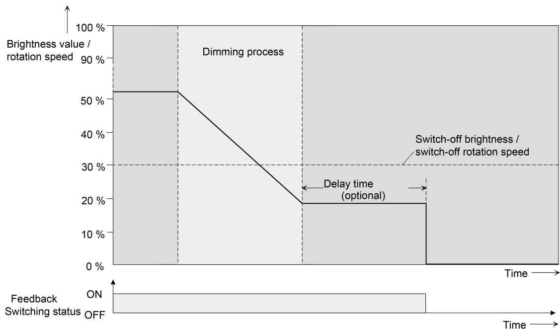
Figure 20: Dimming and switching behaviour of the automatic switch-off function
