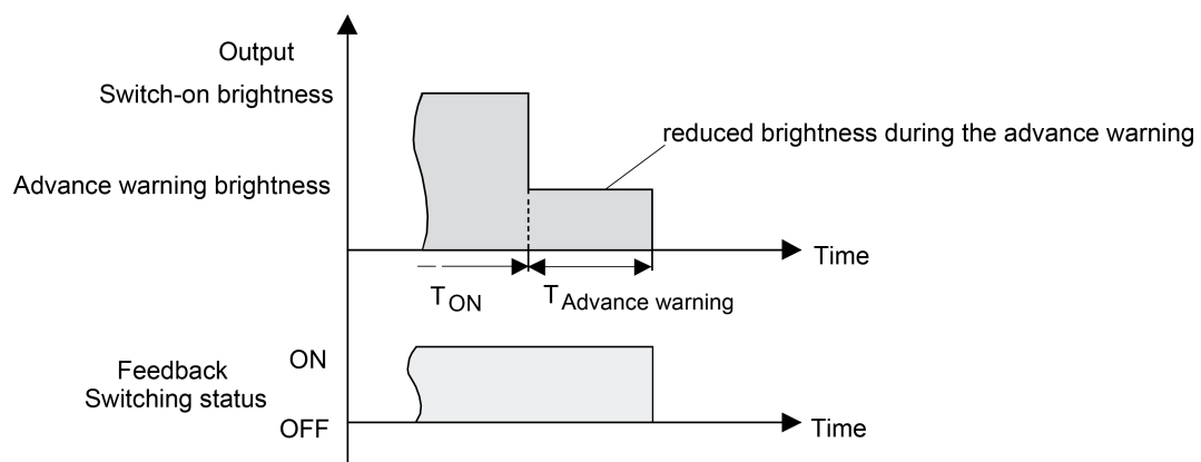
Figure 25: The pre-warning function of the staircase function without soft OFF function
