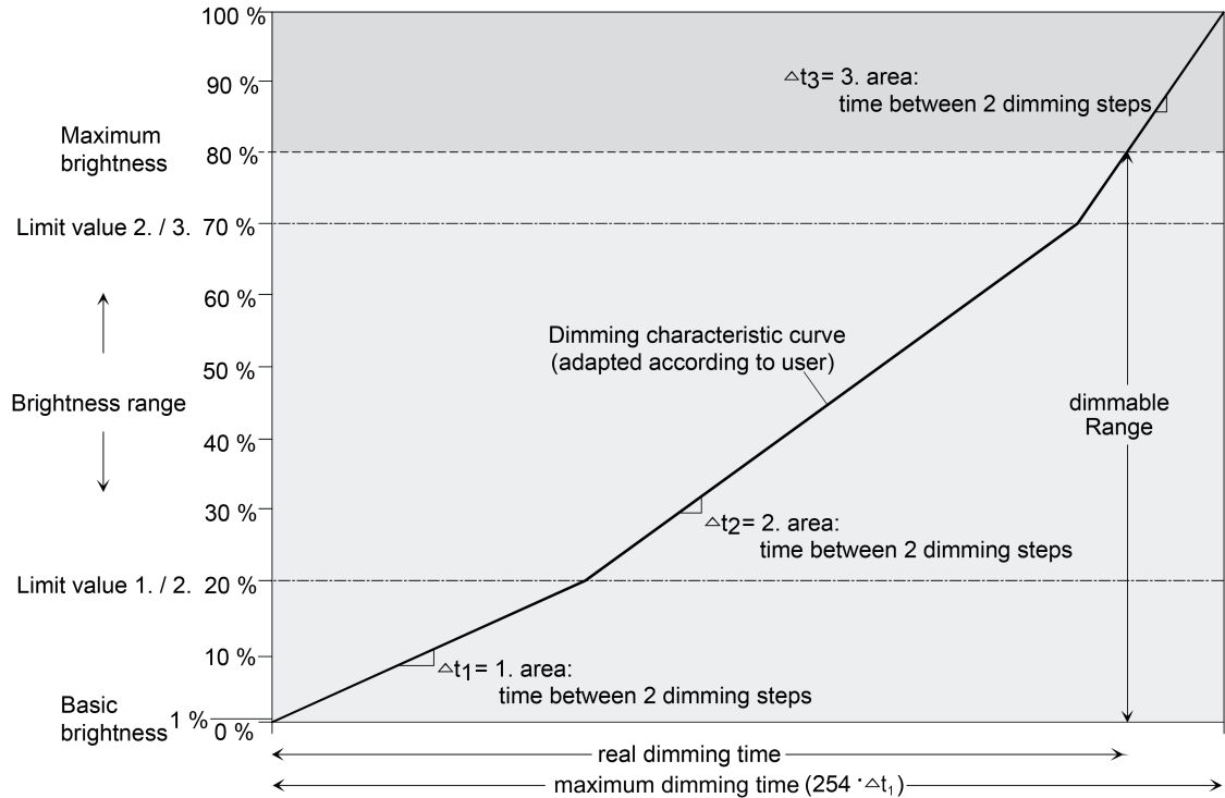
Figure 17: User-defined dimming characteristic as an example with basic brightness and maximum brightness (example with 3 areas)
