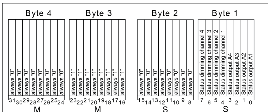
Figure 9: Object structure of the collective feedback
