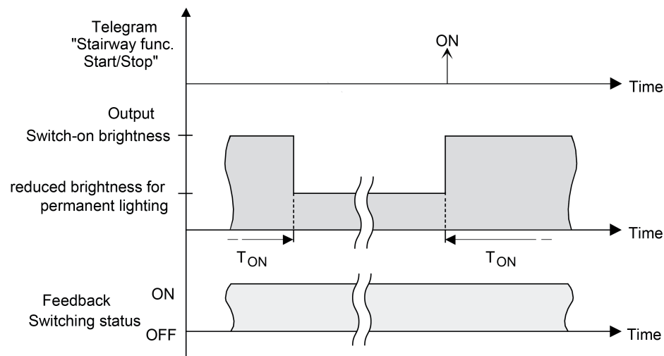
Figure 27: The continuous lighting of the staircase function without soft functions
