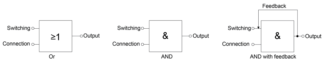
Figure 30: Logic operation types of the logic operation function
