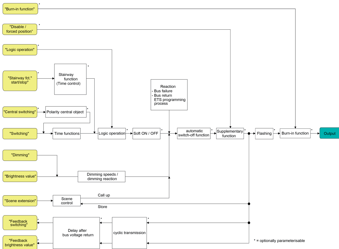
Figure 10: Function diagram of the dimming channels
