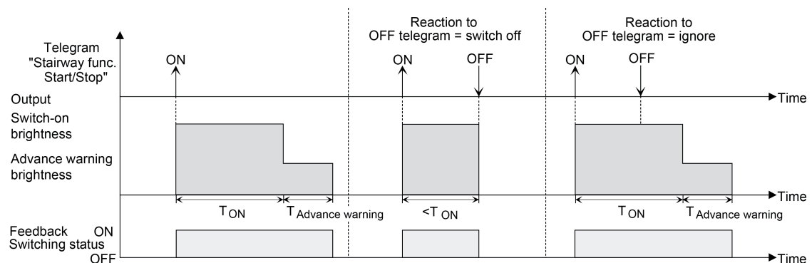
Figure 23: Switch-off behaviour of the staircase function without soft functions
