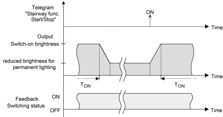
Figure 28: The continuous lighting of the staircase function with soft OFF functions
