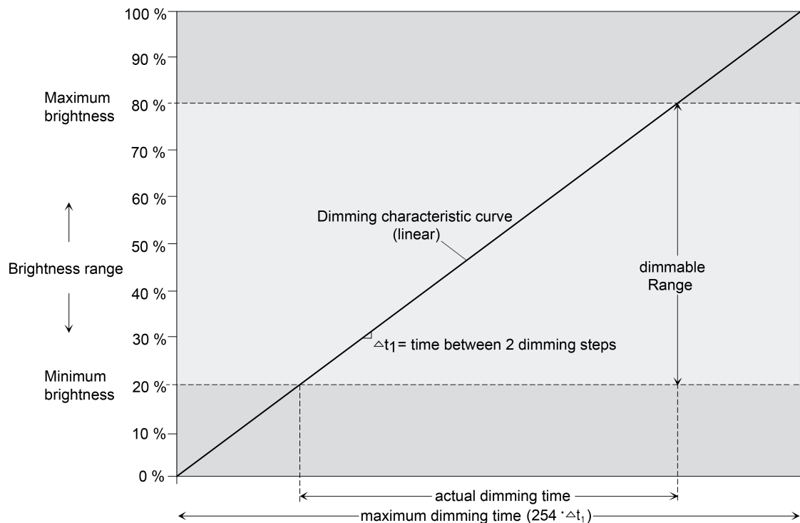
Figure 16: Linear characteristic dimming curve as an example with minimum brightness > 0 % and maximum brightness
