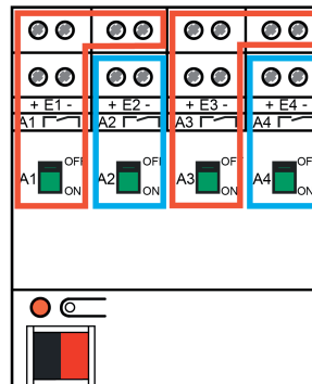
Figure 7: Configuration 4 - Inputs 1 & 2 affect output 1 / Inputs 3 & 4 affect output 3 / Outputs 2 and 4 can be used independently
