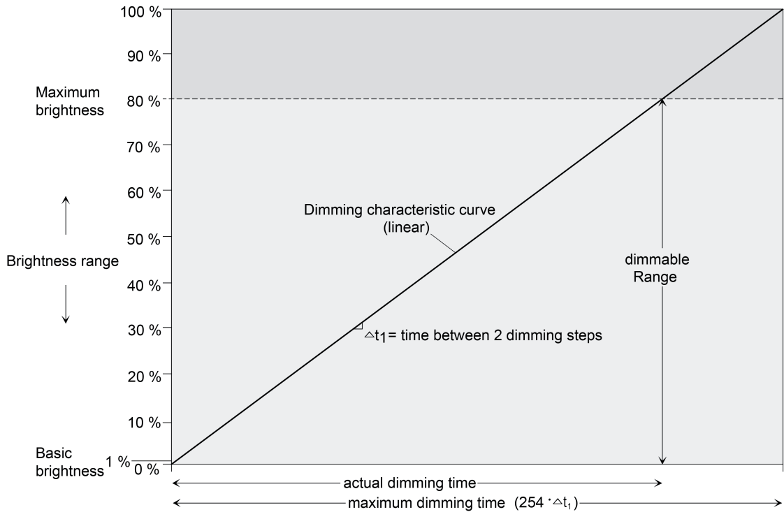
Figure 15: Linear dimming characteristic as an example with basic brightness and maximum brightness
