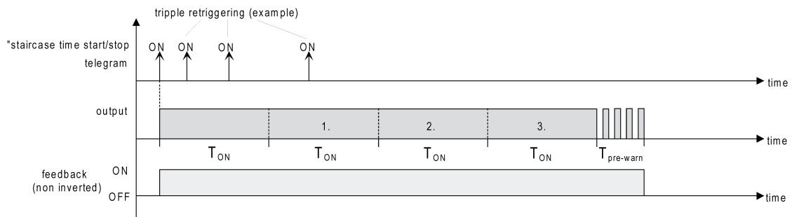
Figure 35: Time extension of the staircase function
