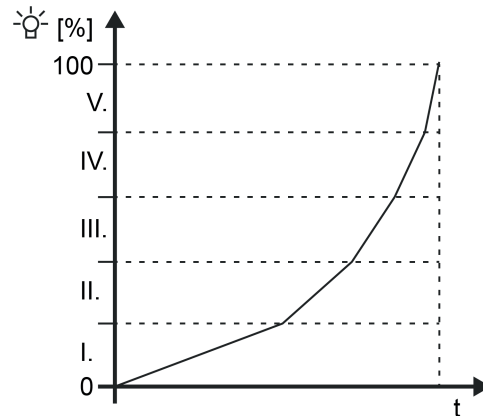
Figure 14: User-defined dimming characteristic (as an example with 5 brightness areas)
