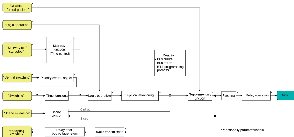
Figure 31: Function diagram of the switching channels
