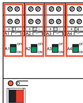
Figure 4: Configuration 1 - Classic application / inputs have a separate effect on the outputs
