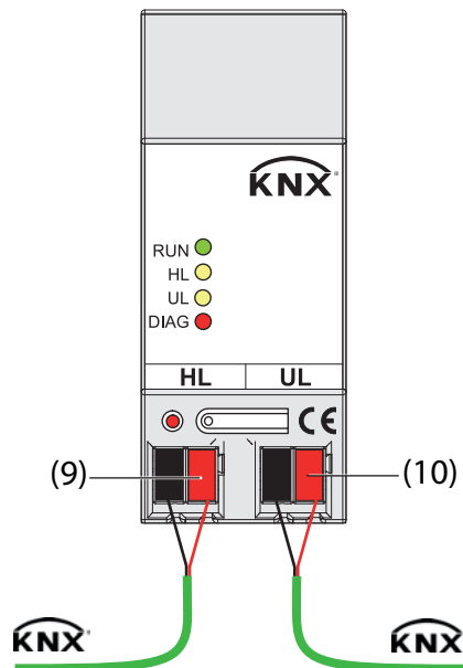
Figure 2: Connection diagram
