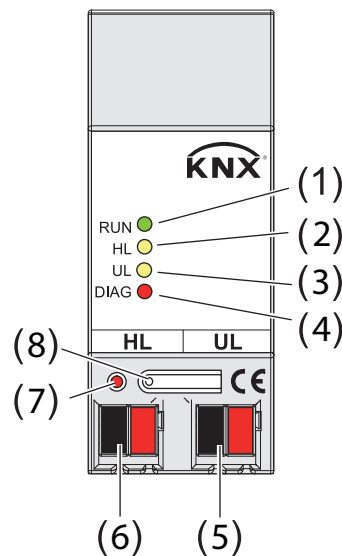
Figure 1: Device components
