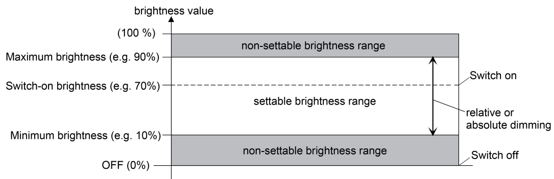
Figure 33: Example of a brightness range with switch-on brightness
