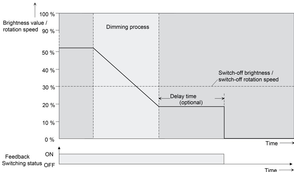
Figure 37: Dimming and switching behaviour of the automatic switch-off function
