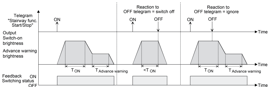
Figure 42: Switch-off behaviour of the staircase function with soft functions (as an example with minimum brightness = 0 %)
