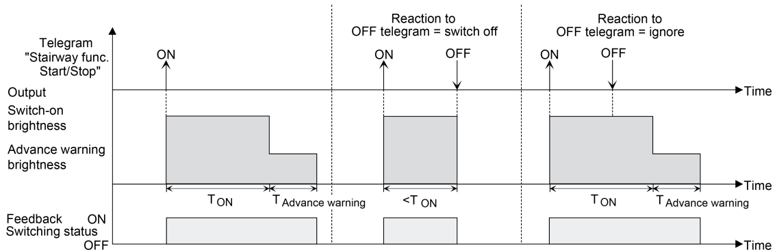
Figure 41: Switch-off behaviour of the staircase function without soft functions
